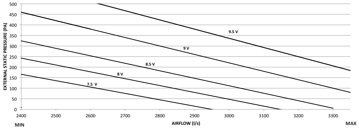
FAN PERFORMANCE CURVE S055IHR3SA-
