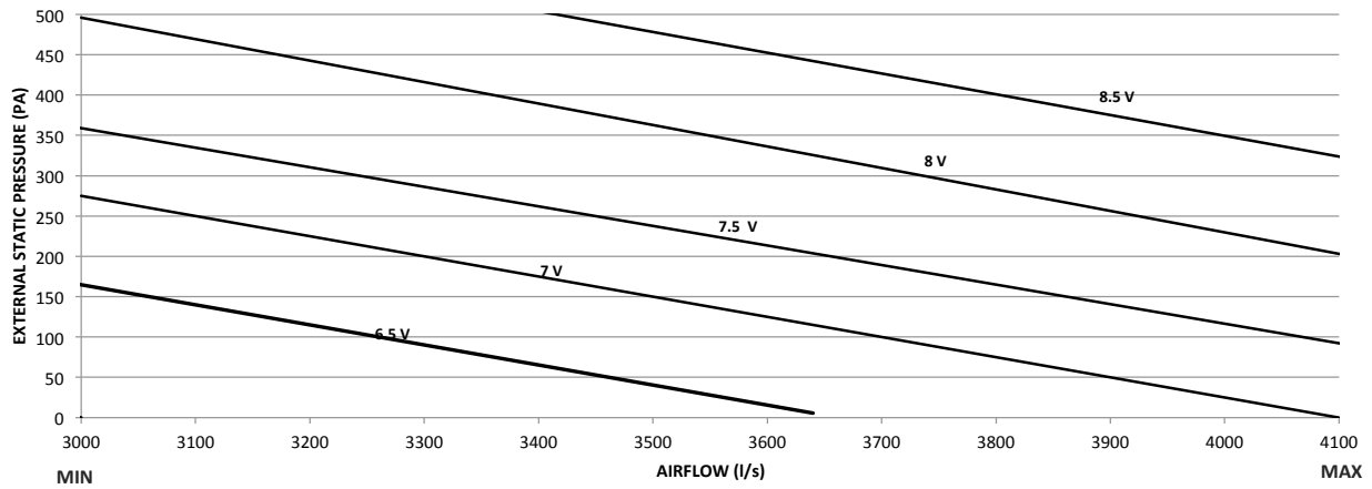
FAN PERFORMANCE CURVE P065AHR3SA-
