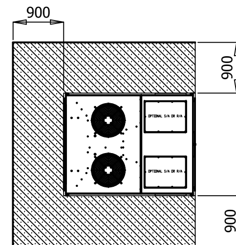
CLEARANCE DETAIL
