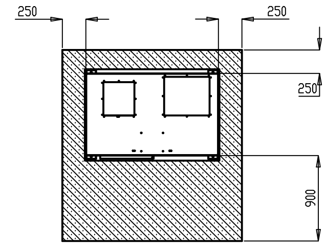
CLEARANCE DETAIL
