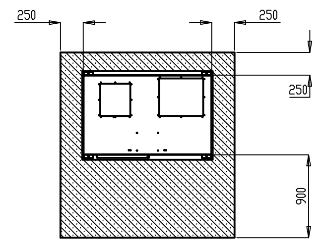
CLEARANCE DETAIL
