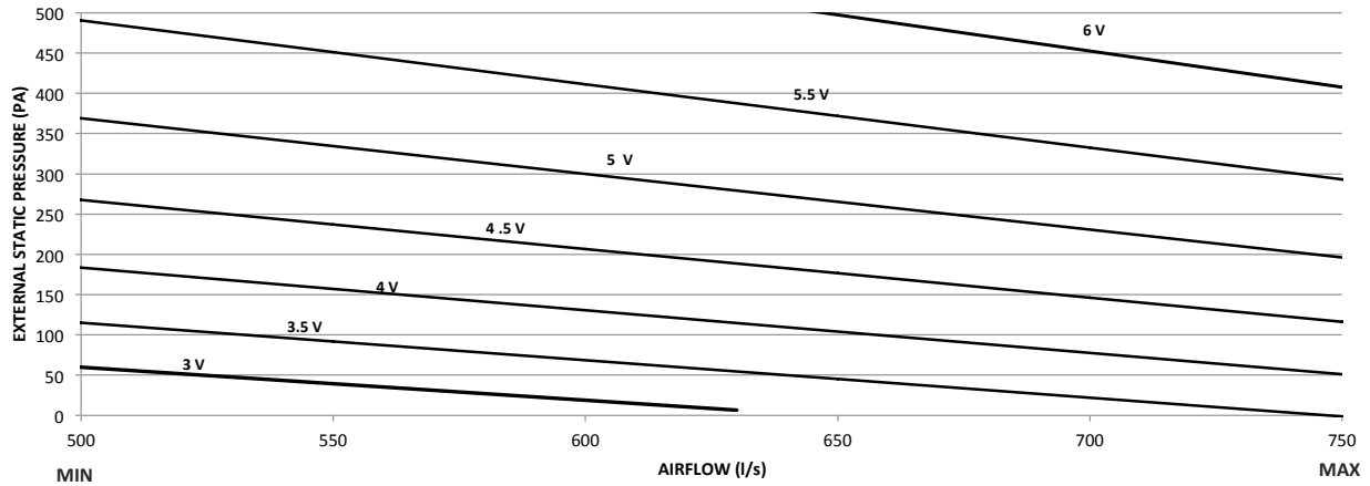
FAN PERFORMANCE CURVE P012AVR3SA-
