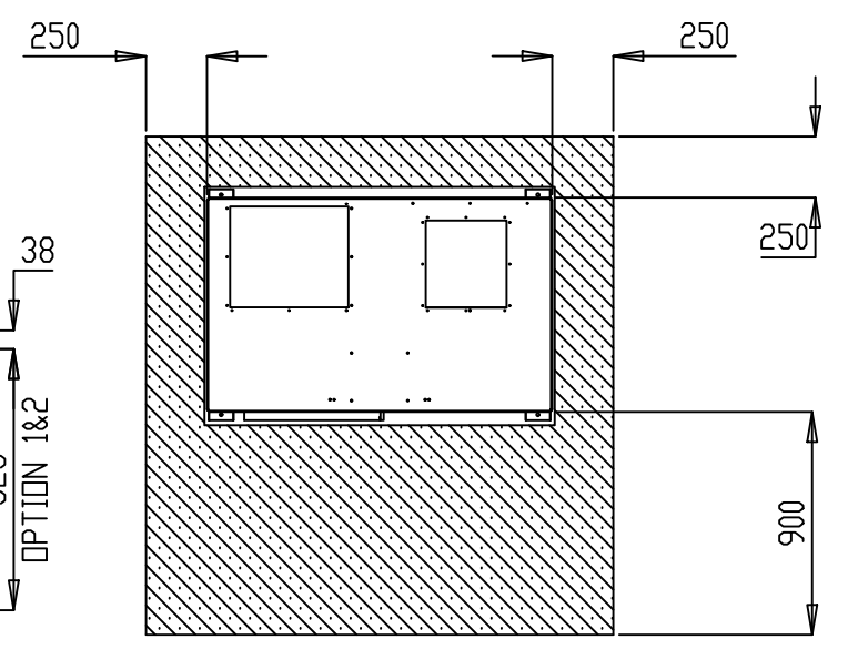
CLEARANCE DETAIL
